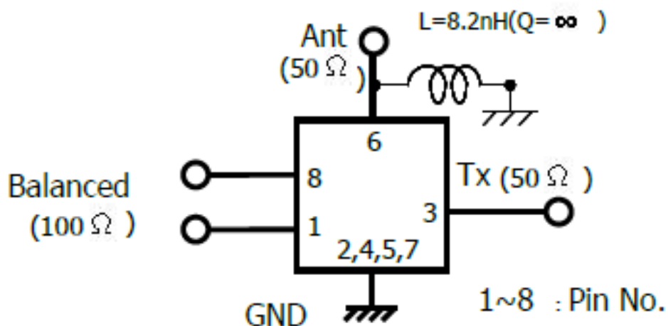
Figure 2. Evaluation Circuit
